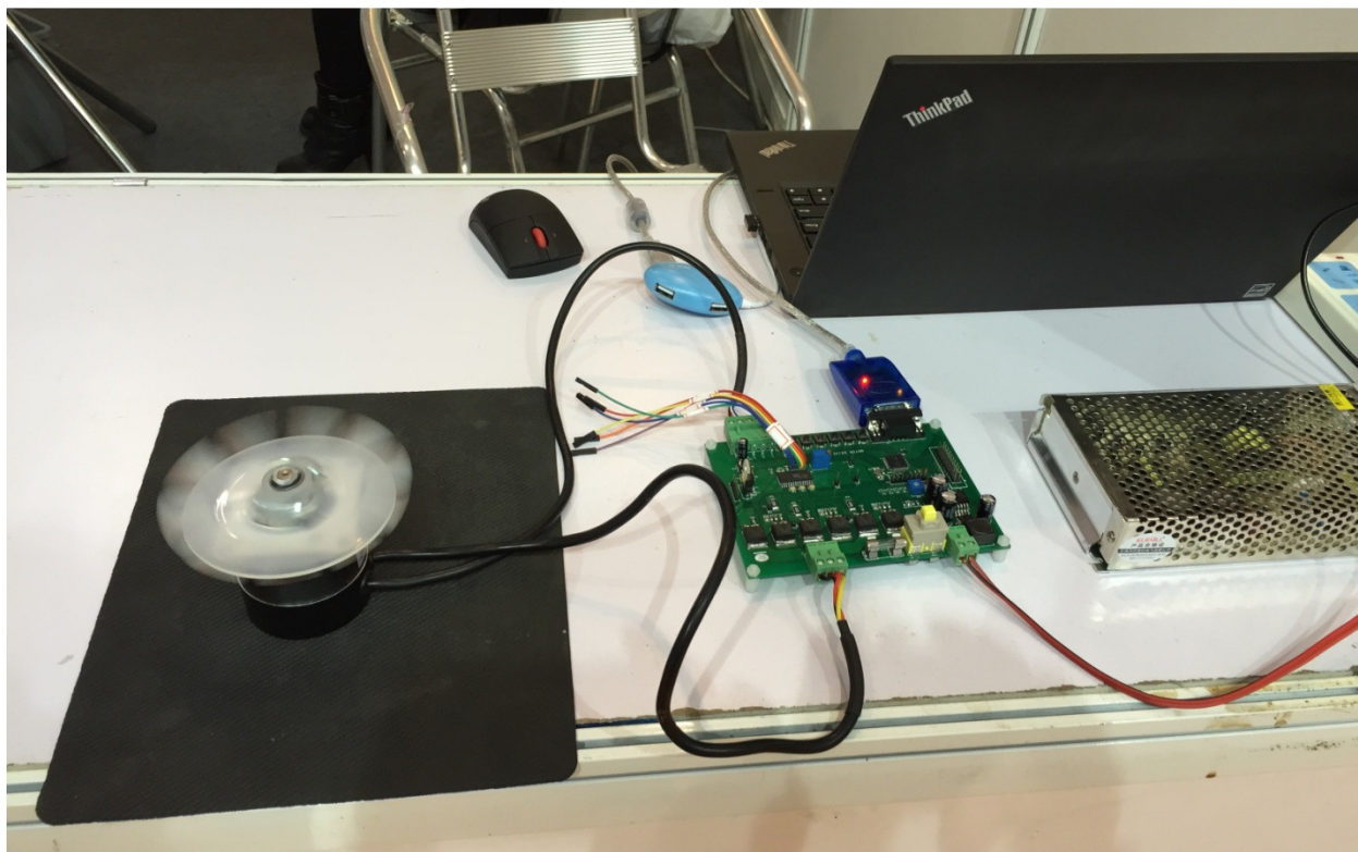
Fig.2 JMT1808 FOC motor controller EVB.
